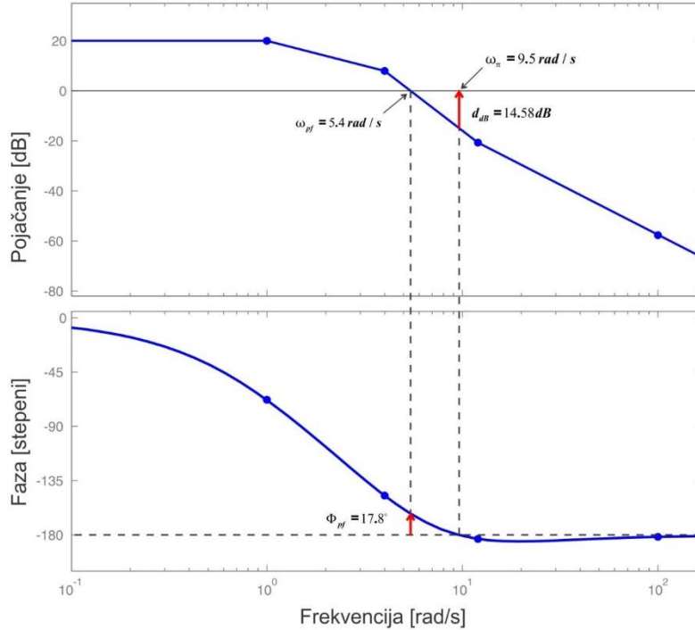
Slika 5 Bodeovi dijagrami, W(s) = \frac{40(s+12)}{3(s+1)(s+4)^2}
